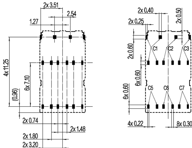
RECOMMENDED PCB LAYOUT (TOP VIEW) GENERAL TOLERANCE: ±0.05
